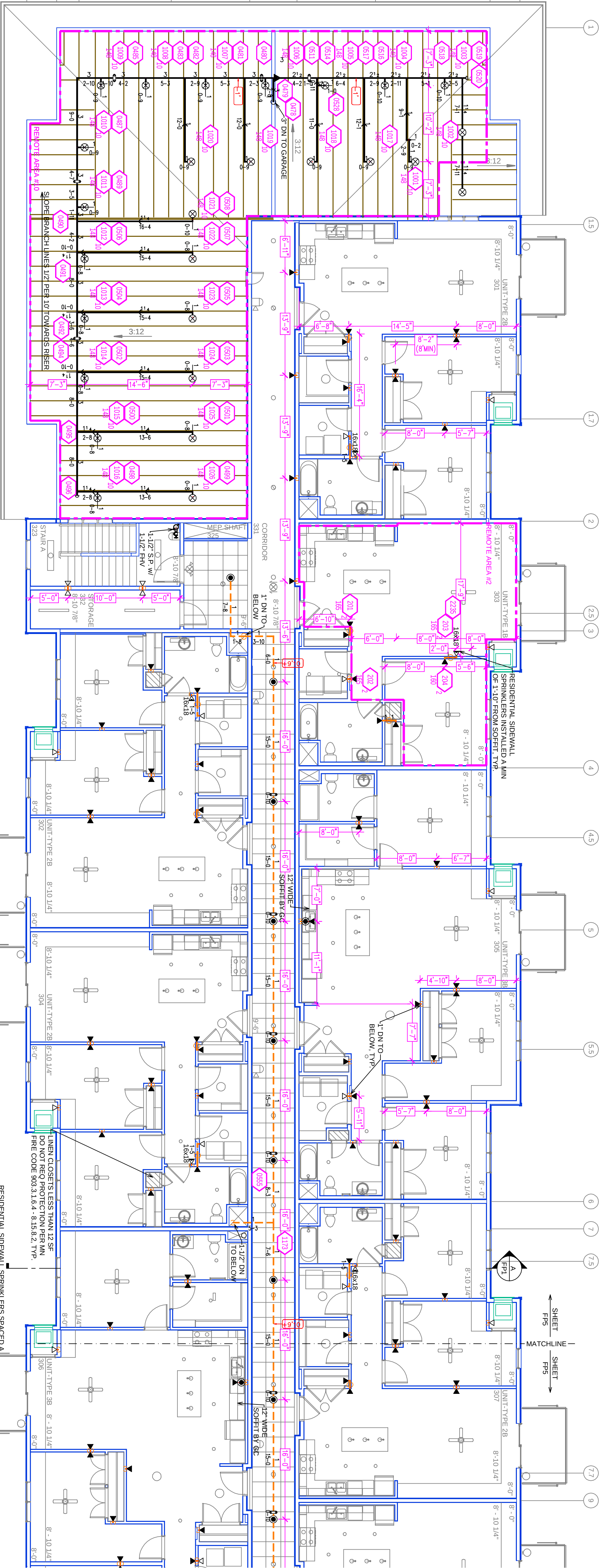
THIRD FLOOR-A FIRE SPRINKLER PLAN SCALE= 1/8" = 1'-0"
