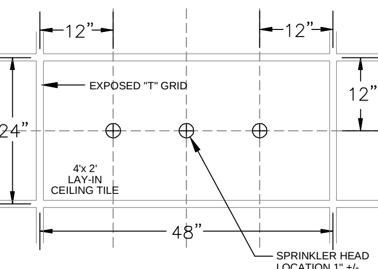
TYP. 4'X2' CENTER OF TILE SPRINKLER HEAD DETAIL N.T.S.
