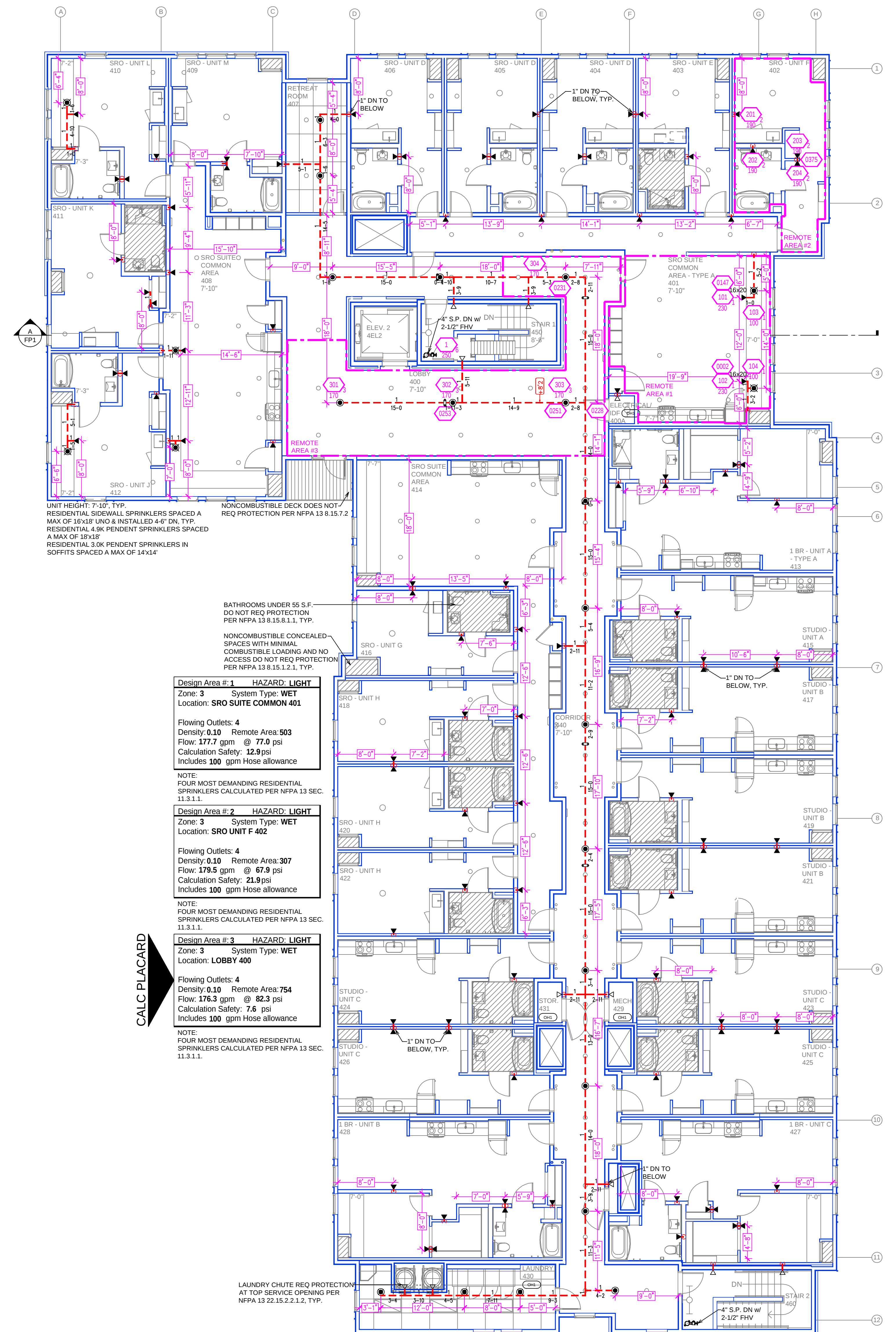
LEVEL 4 FIRE SPRINKLER PLAN SCALE= 1/8" = 1'-0"
