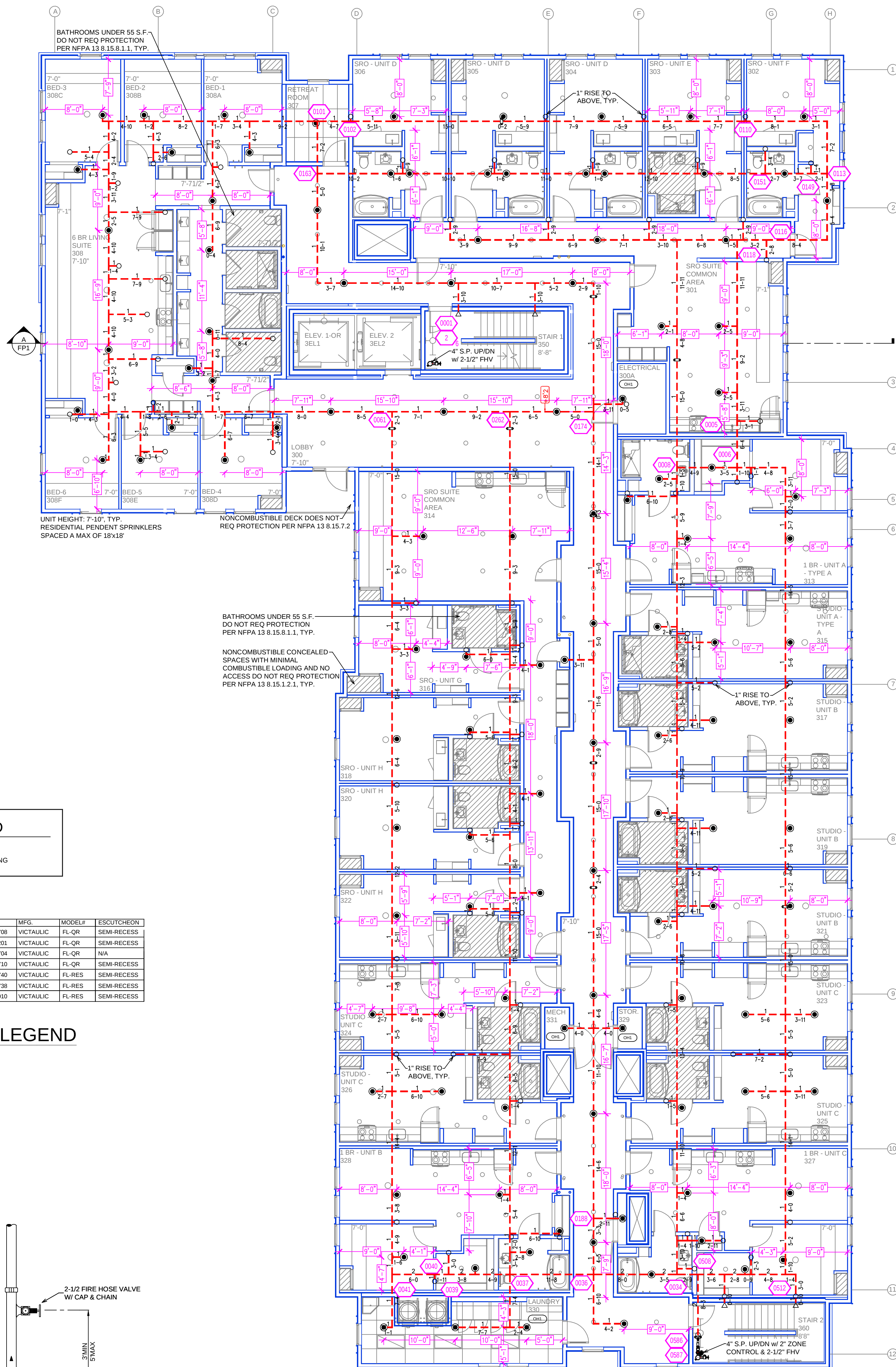
LEVEL 3 FIRE SPRINKLER PLAN SCALE= 1/8" = 1'-0"
